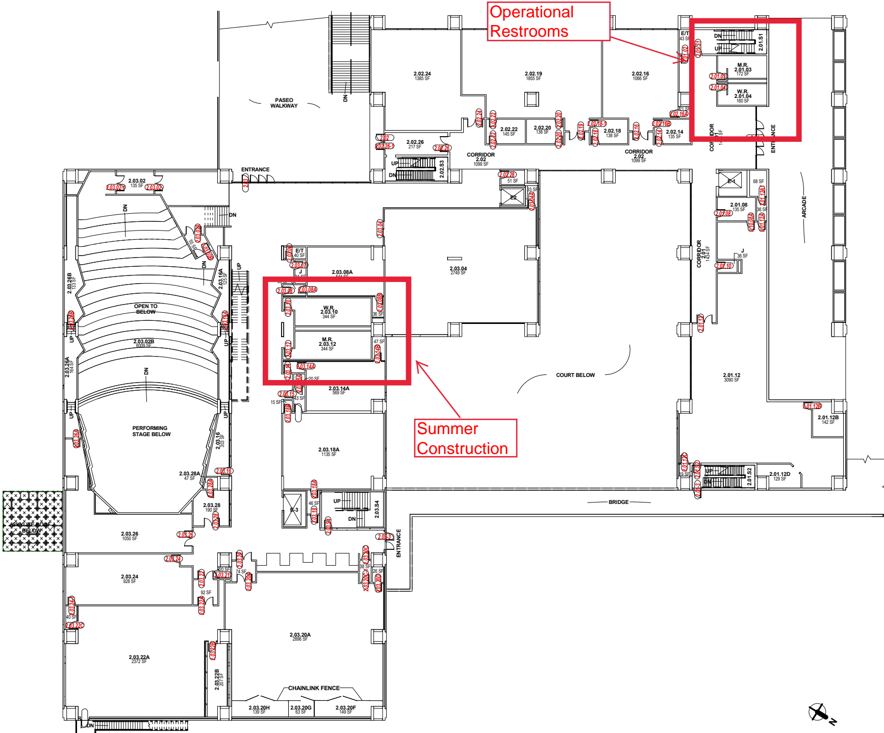
1 Floor Plan Level 2 SCALE: NTS
